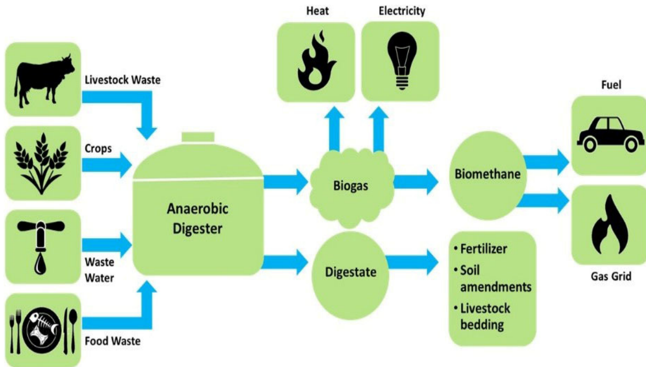
Figure 1: Anaerobic digestion process
